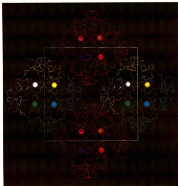
Fig. 1. The Hall anions (represented by solid spheres) at molecular interfaces in the tetragonal lysozyme crystal as viewed on the ab plane. These anions hold together the molecules forming the 4_3 helices. The square represents the unit cell. The anions and protein molecules are made different colours only to assist in distinguishing them.
